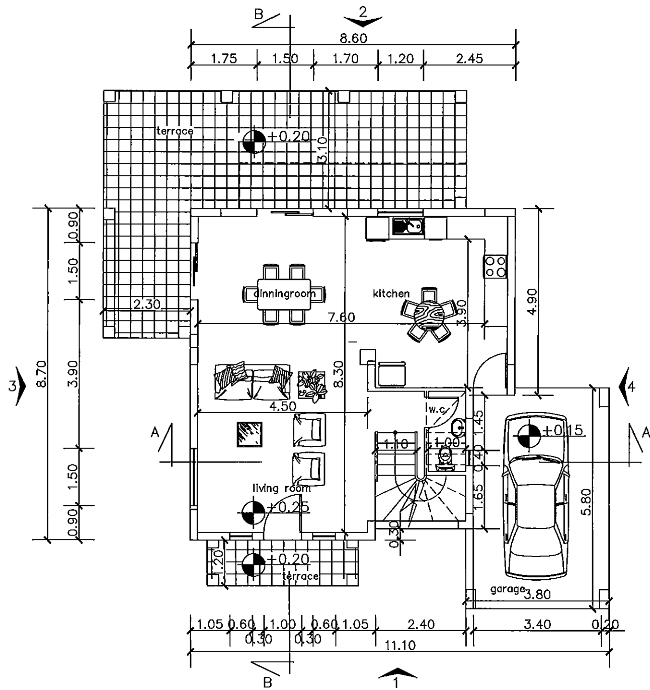
GROUND FLOOR
