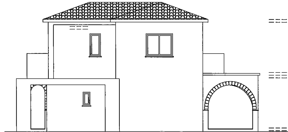
ELEVATIONS 4
